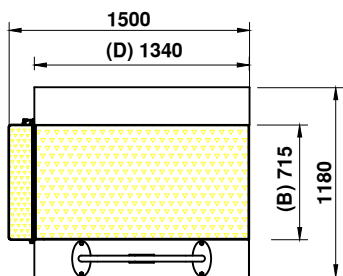
Low-Up platform afmeting: (BxD) 715 x 1340
